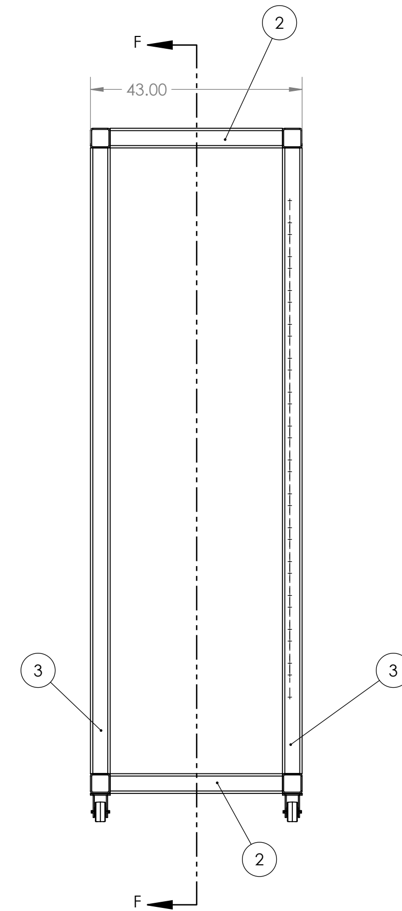
END VIEW SCALE 1:20
