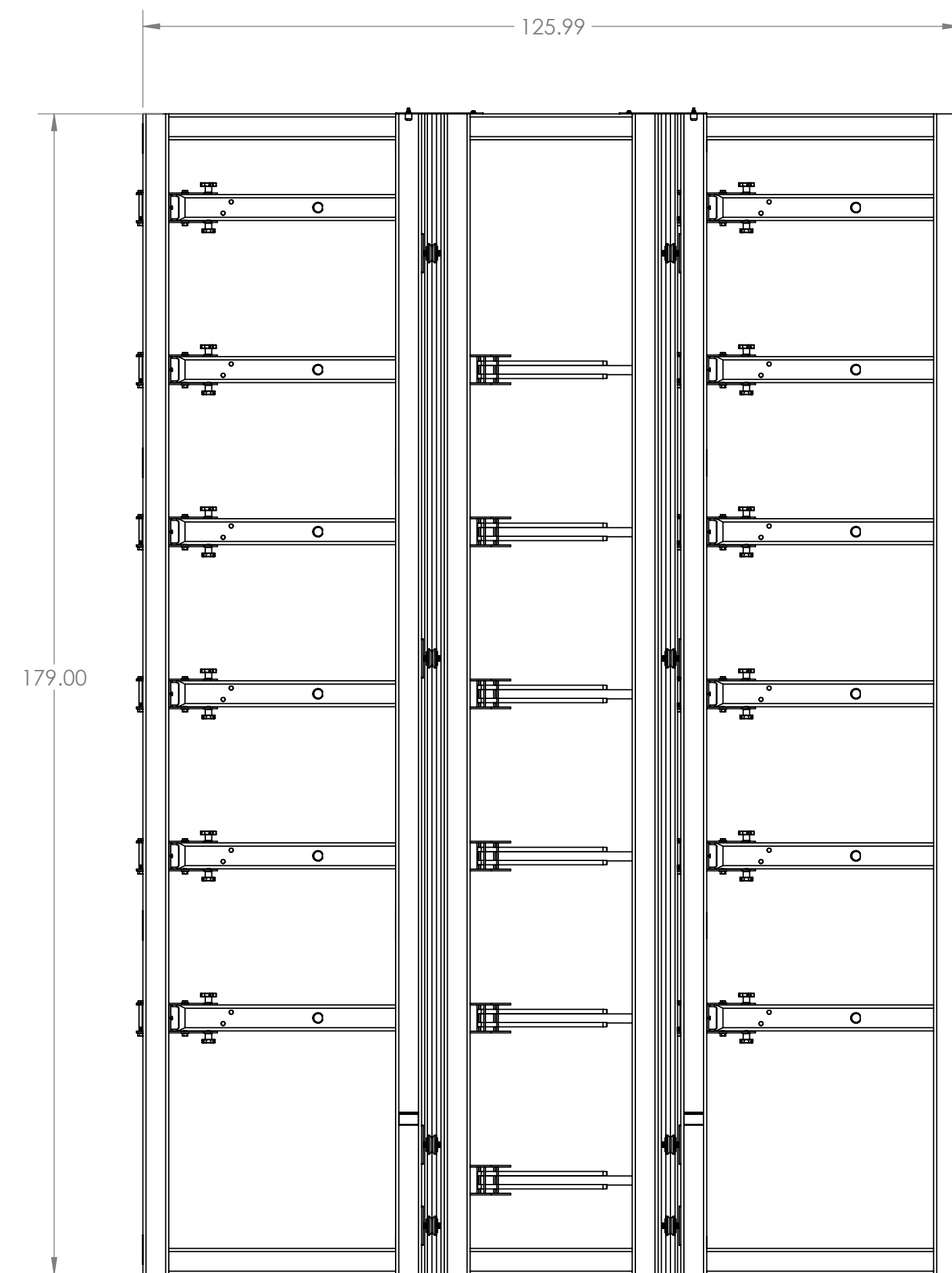
PLAN SCALE 1:20
