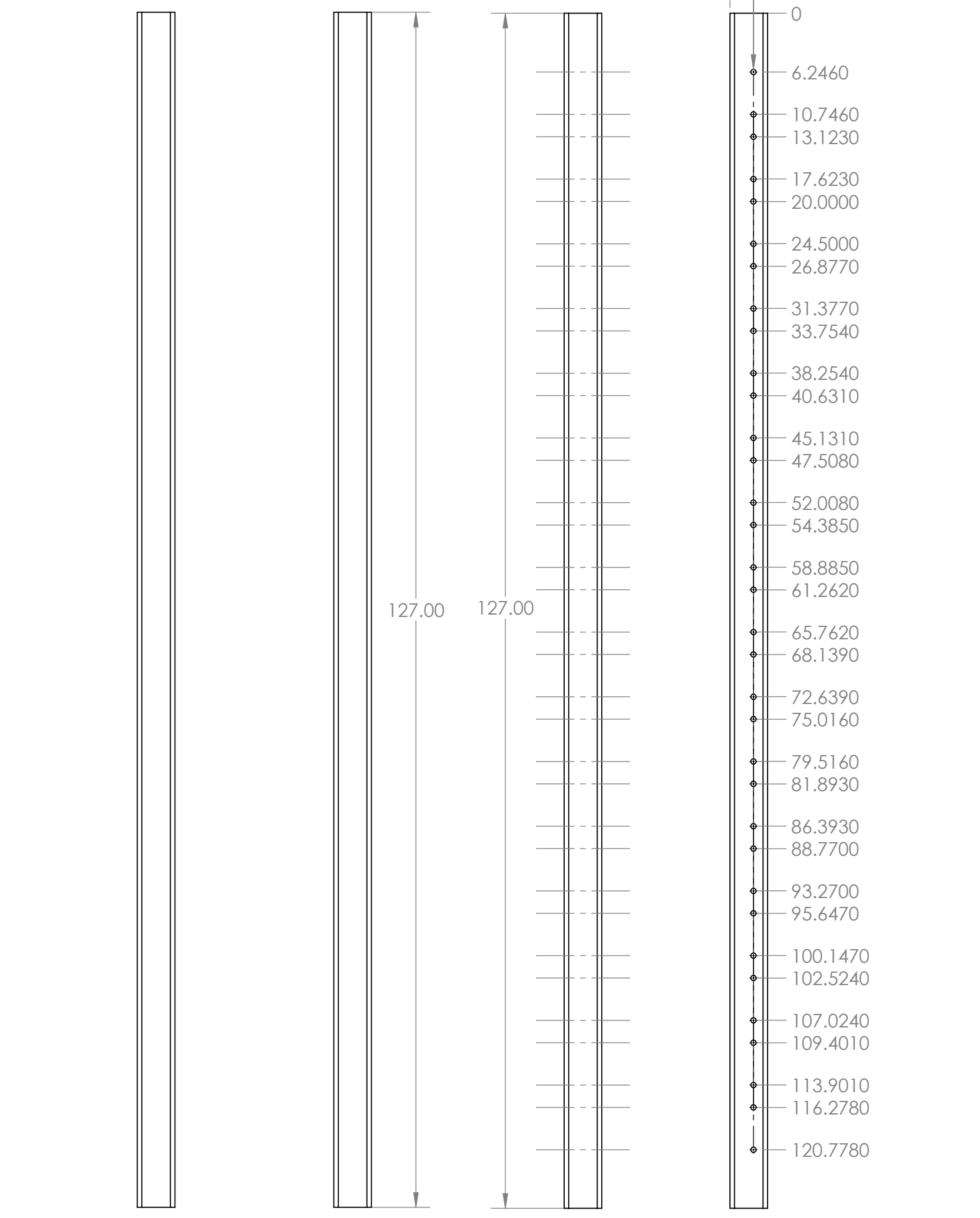
3 DETAIL SCALE 1:12 SIDE VIEW SCALE 1:12 4 DETAIL SCALE 1:12 SIDE VIEW SCALE 1:12
