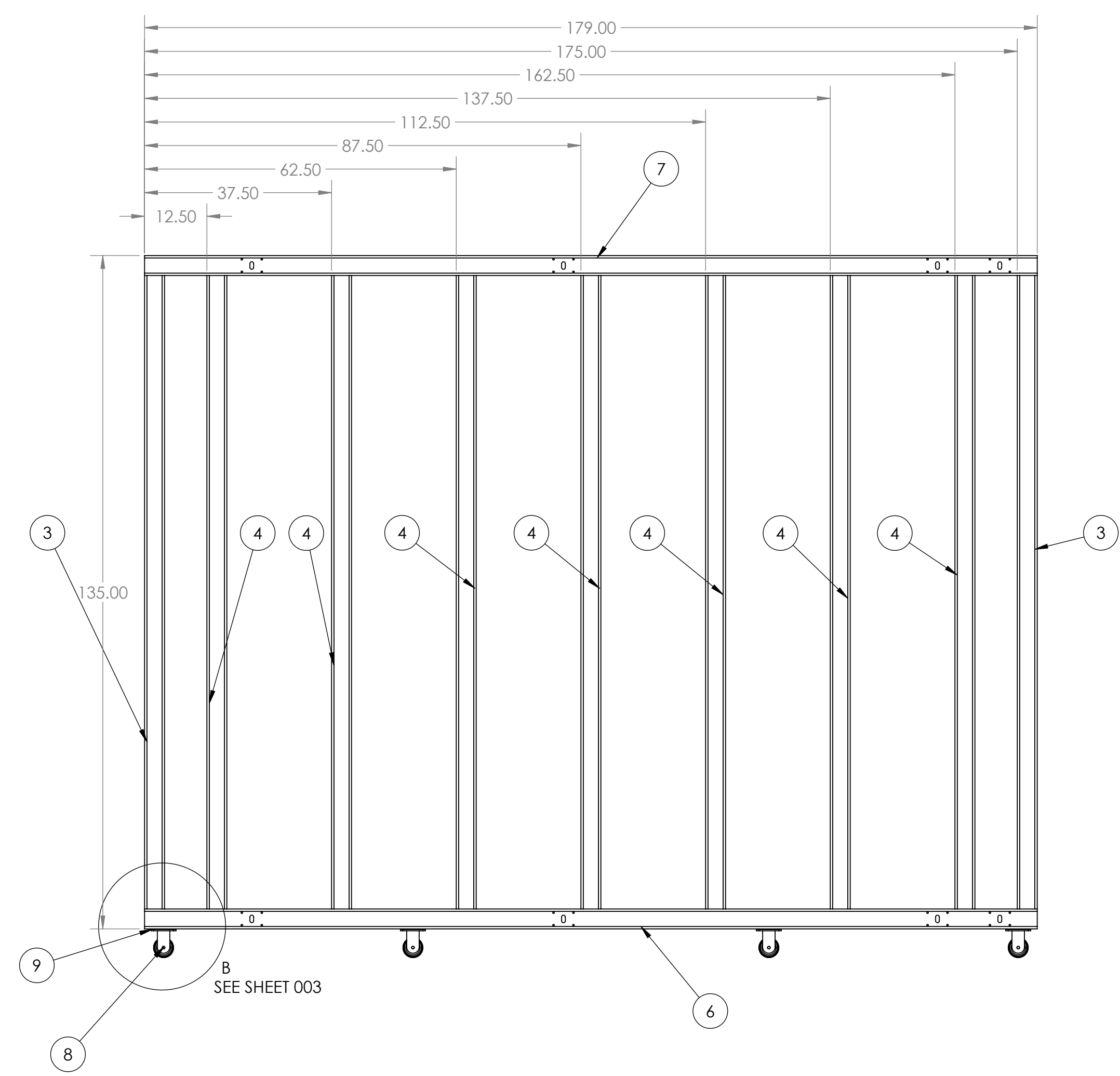
SIDE VIEW SCALE 1:20
