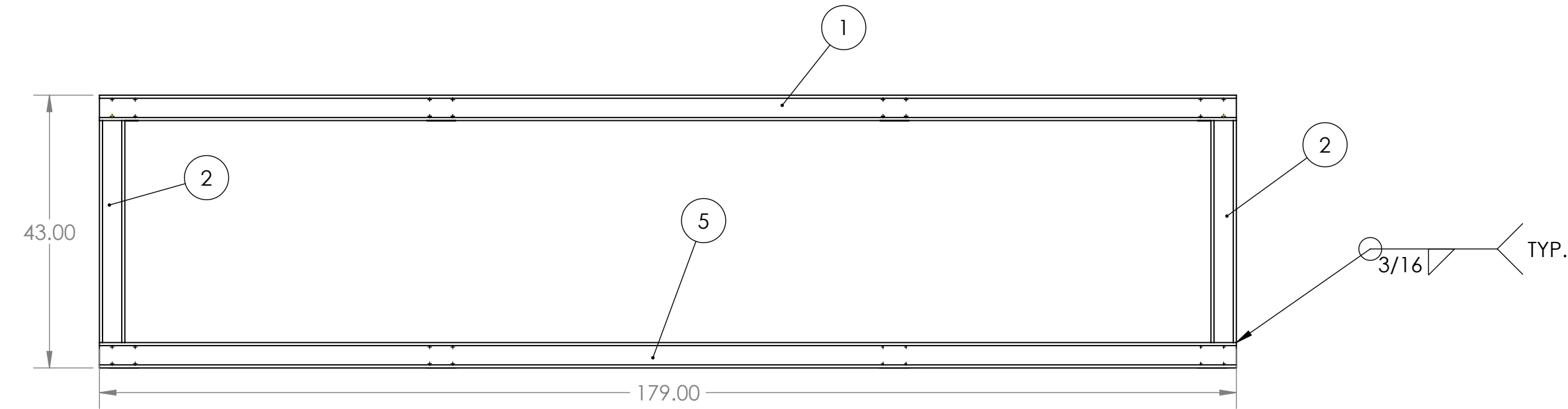
PLAN SCALE 1:20
