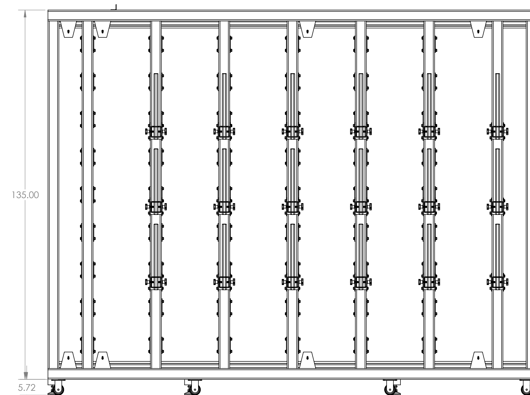
SIDE VIEW SCALE 1:20
