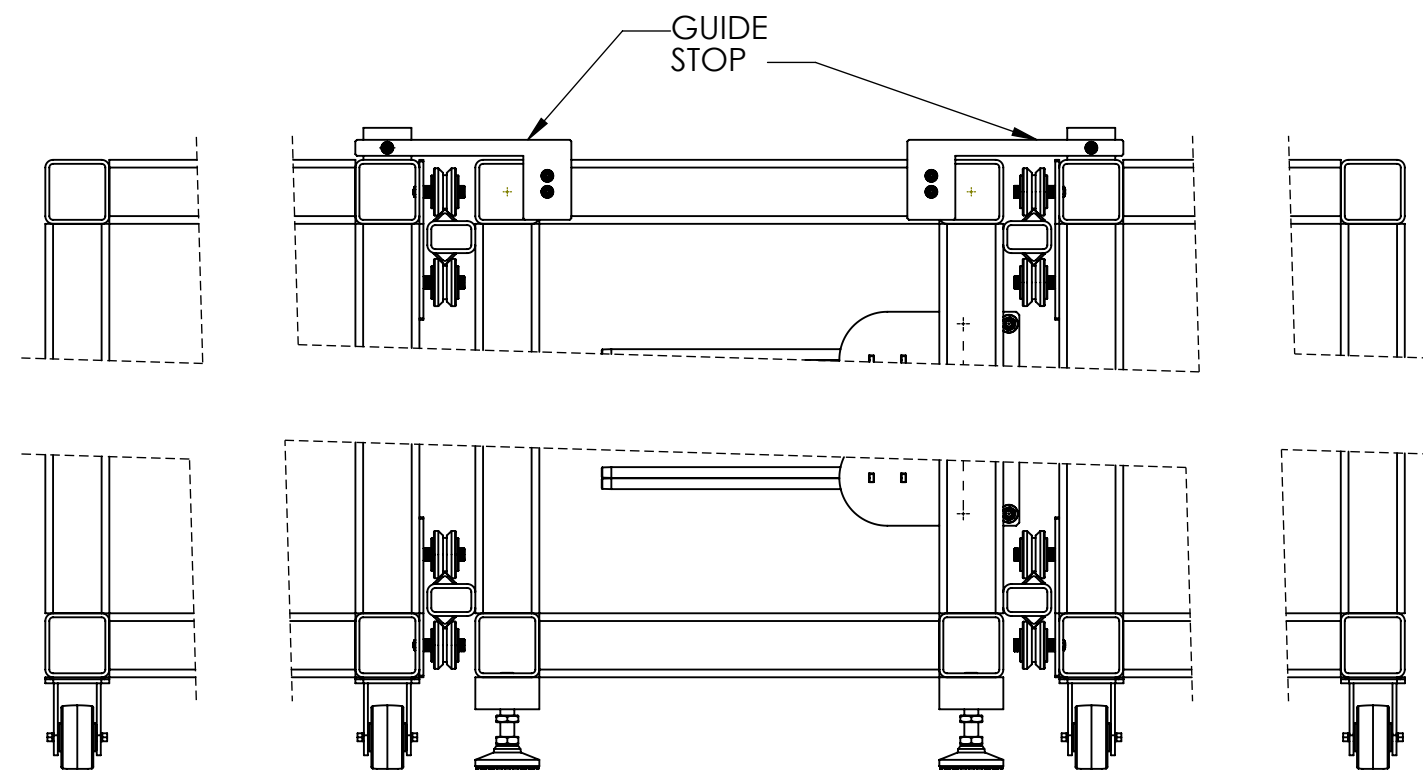
FULL ASSEMBLY FRONT VIEW SCALE 1:12
