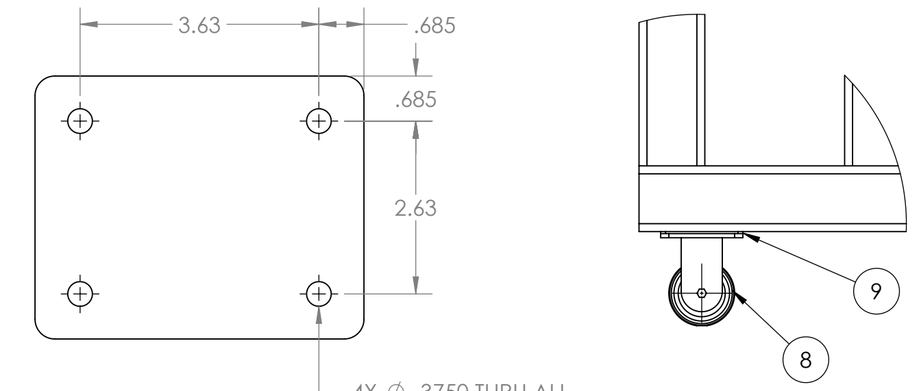
PLAN SCALE 1:2 DETAIL B SCALE 1:8
