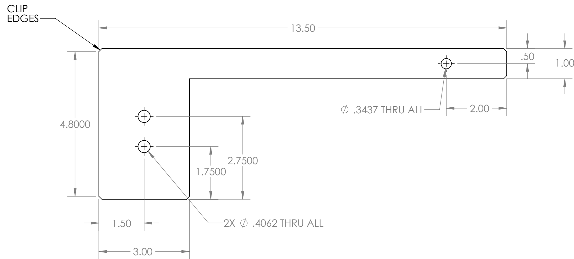
1 DETAIL SCALE 1:2
