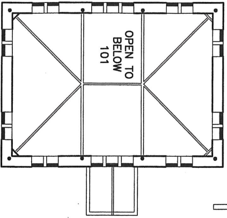
CLEARSTORY PLAN
