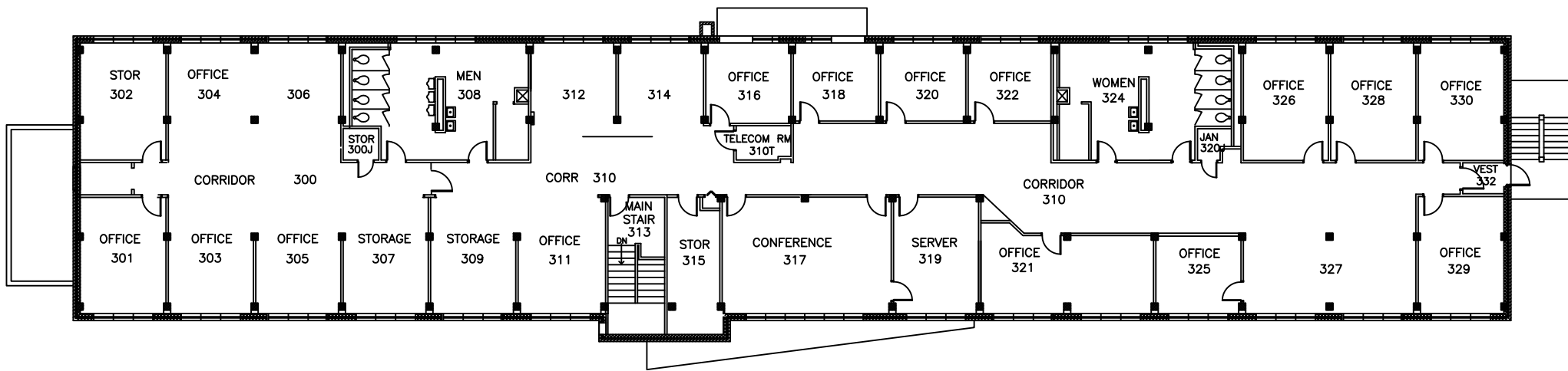
THIRD FLOOR PLAN
