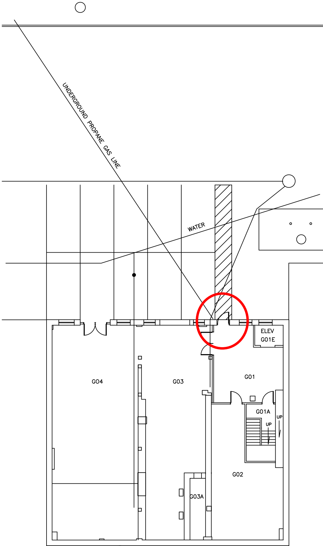
PARKING & LOWER LEVEL II PLAN GANNETT BUILDING 331 WATER STREET UNIVERSITY OF MAINE AT AUGUSTA
