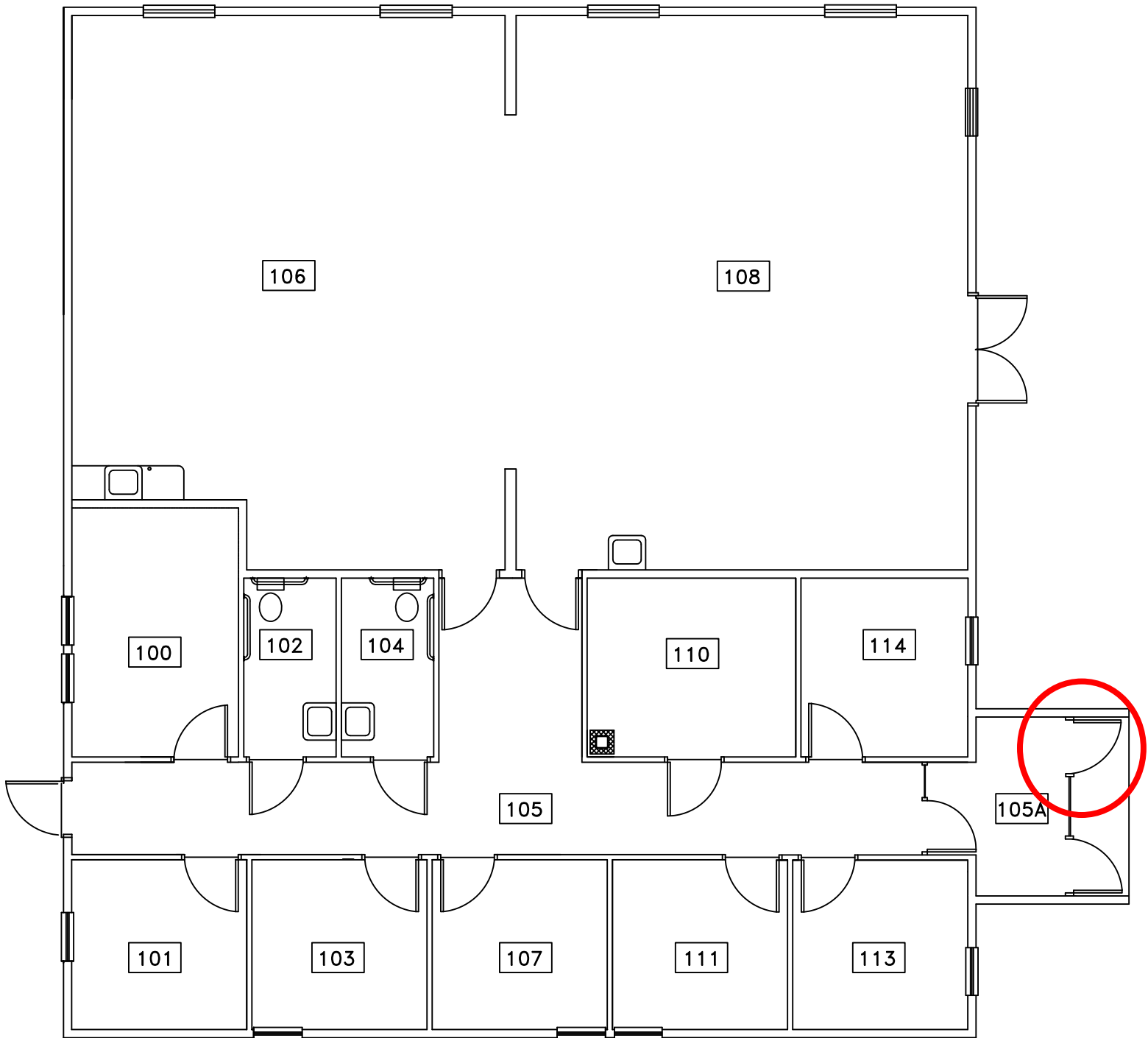
ART AND ARCHITECTURE BUILDING UNIVERSITY of MAINE at AUGUSTA
