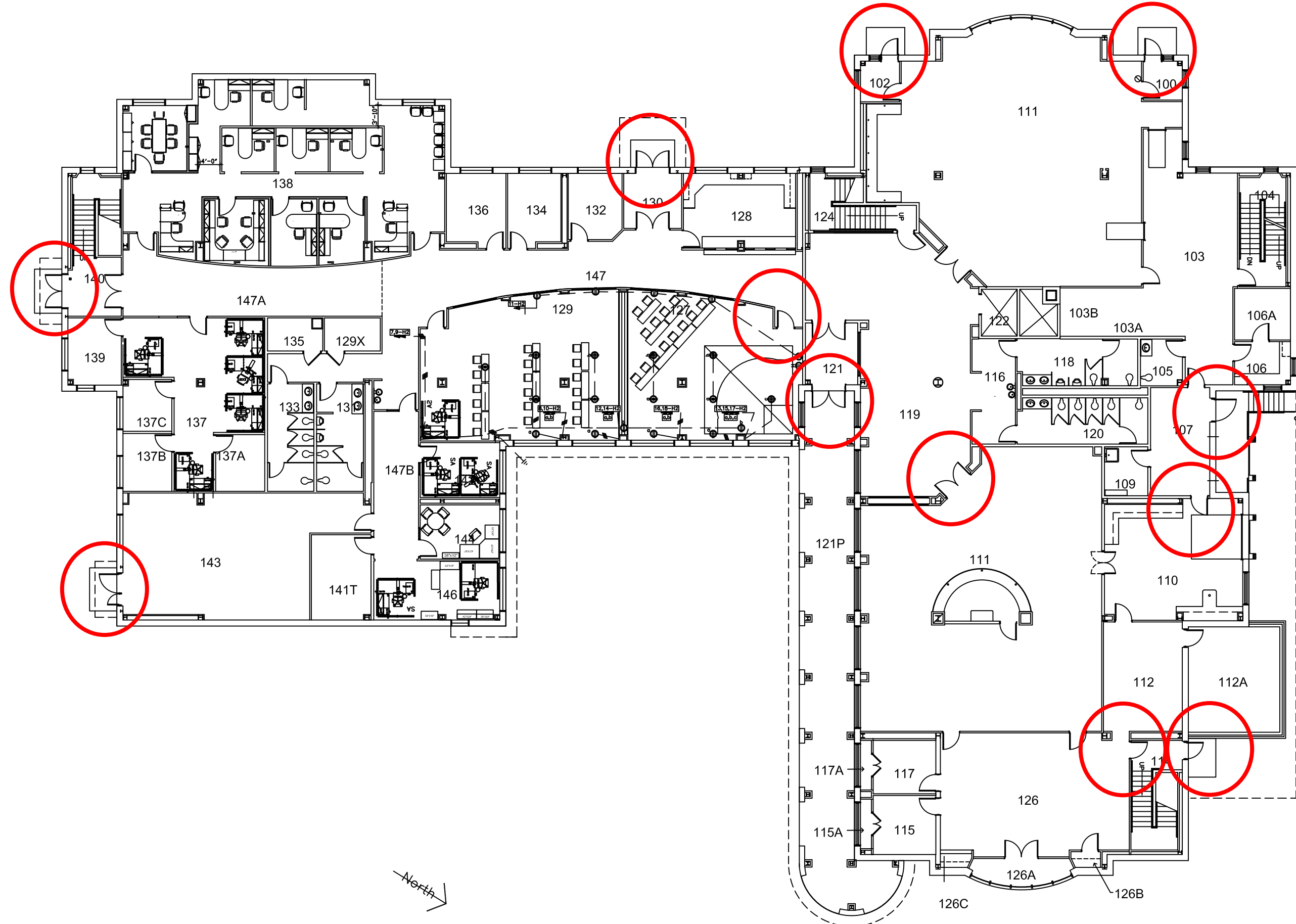
FIRST FLOOR PLAN STUDENT TECHNOLOGY CENTER UNIVERSITY OF MAINE AT AUGUSTA
