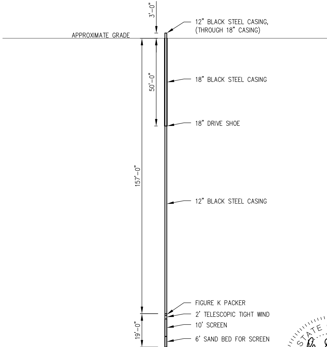
IRRIGATION WELL SCALE: 1/32 = 1'-0"
